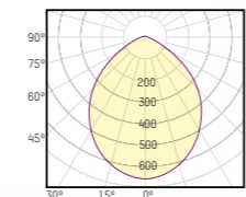
MIKROPRISMATISCHE ABDECKUNG MICROPRISMATIC COVER
